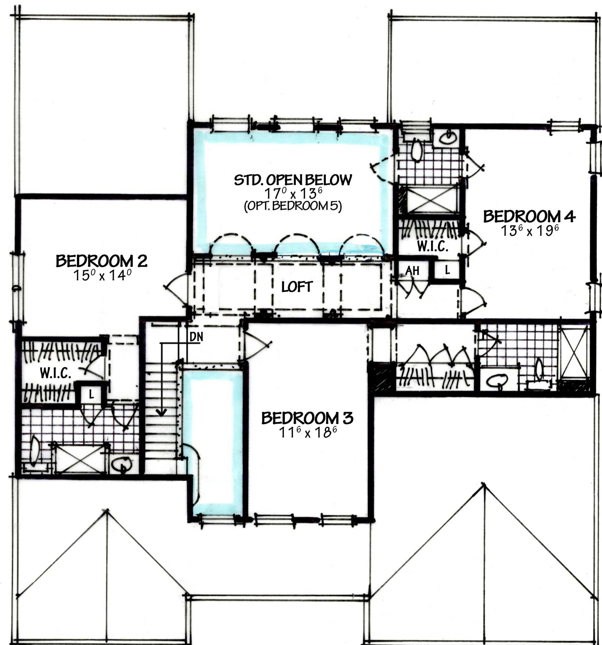
SECOND FLOOR PLAN S.F. 1,288 SCALE: 1' = 1/8"
