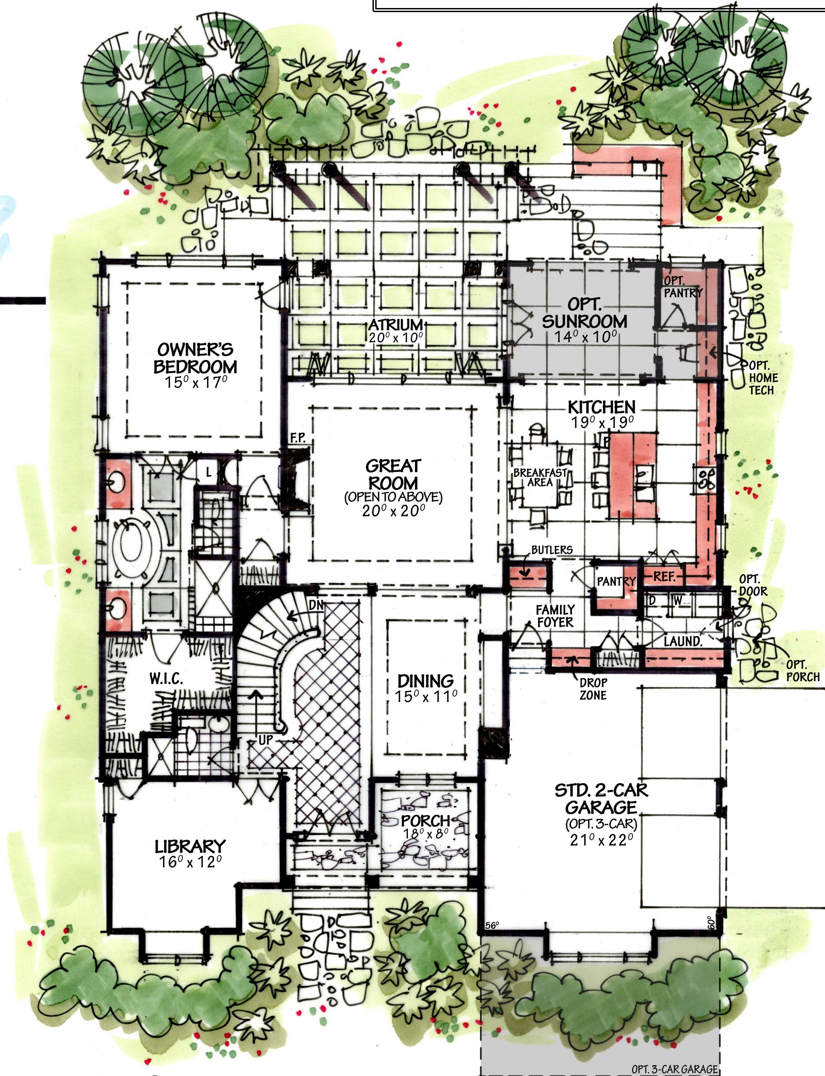
FIRST FLOOR PLAN S.F. 2,282 SCALE: 1' = 1/8"
